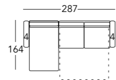
0TOGC3 (1TOGD2M1EP - 1TOGDORM1 1TOGBRSX4 - 1TOGBRDX4)
